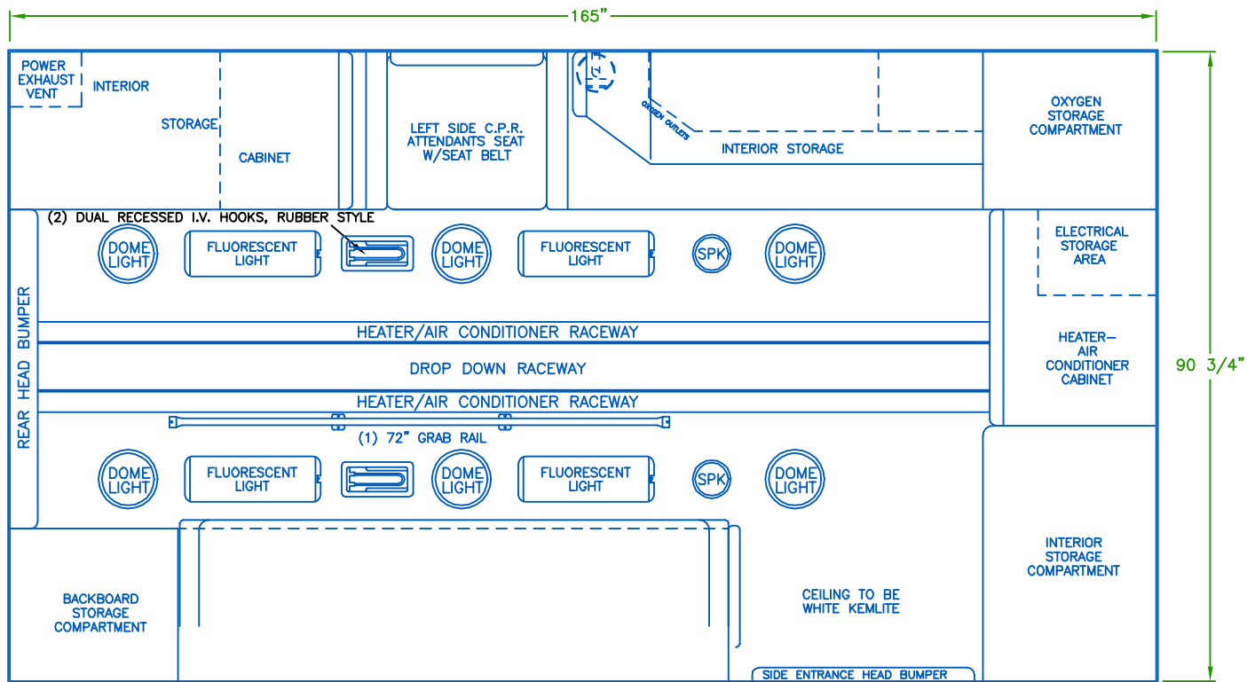
CEILING VIEW
