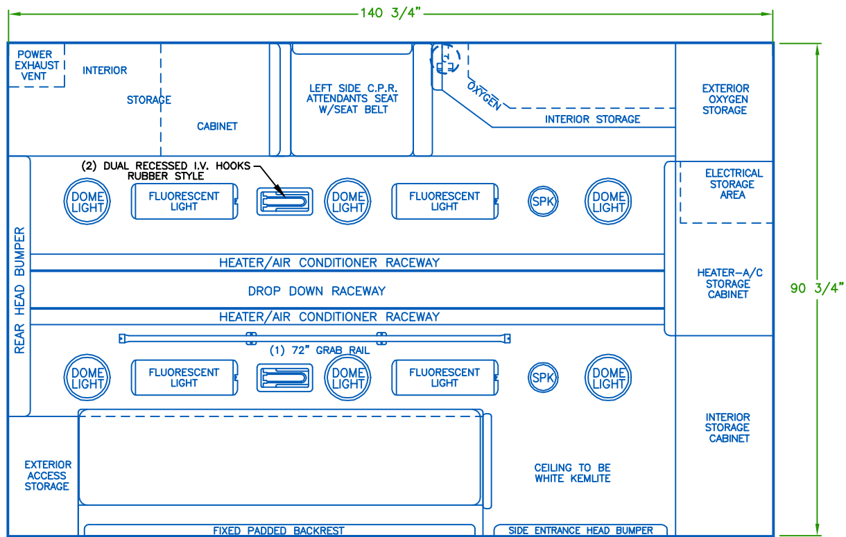
CEILING VIEW
